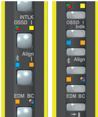
FIG. 8B: LED INDICATORS ON RECEIVER UNIT (30 MM AND 14 MM RESOLUTION)
